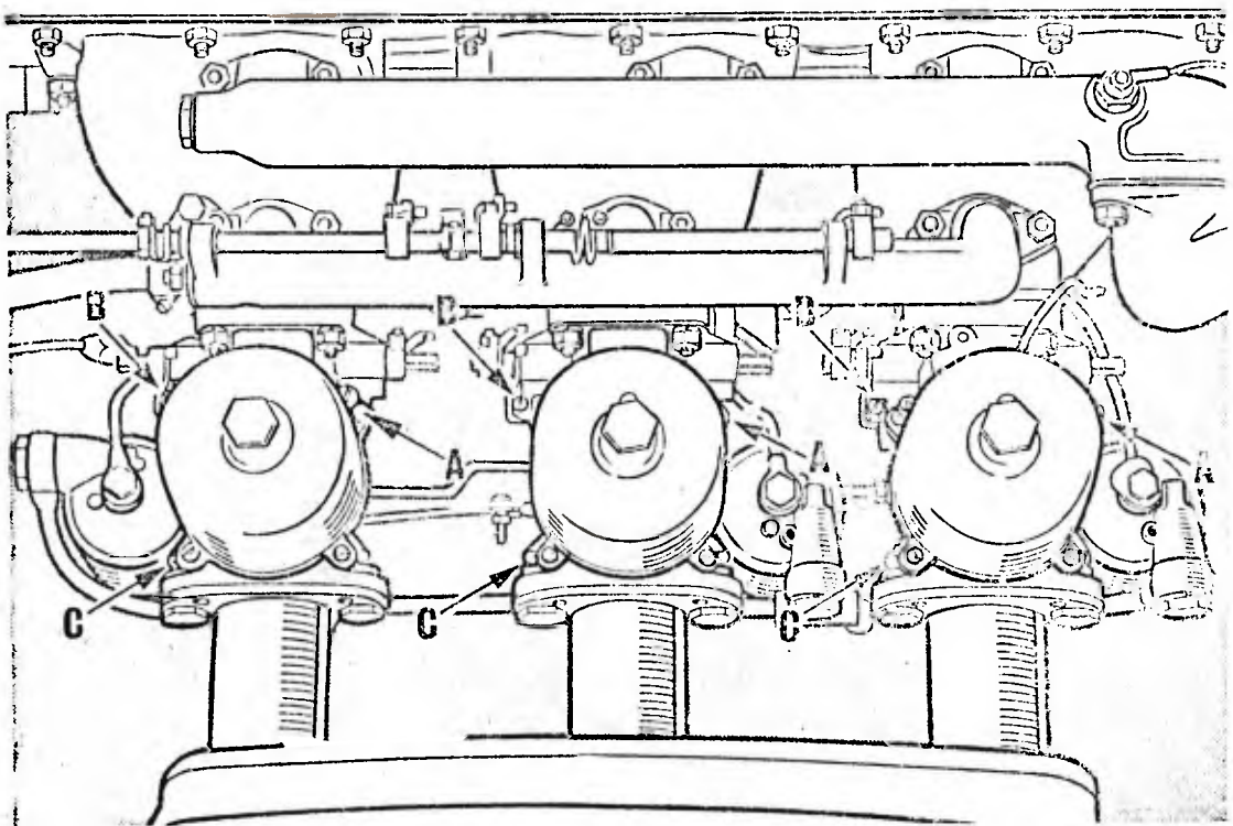
Triple S.U. carburetors are used on the XKE and 4.2 XKE models. (A) Idle speed adjustment, (B) fast-idle speed adjustment, (C) mixture adjustment.
